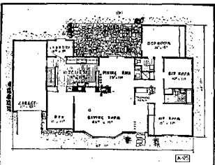
Area: 2,506 sq. ft. Cubage: 25,200 cu. ft.
